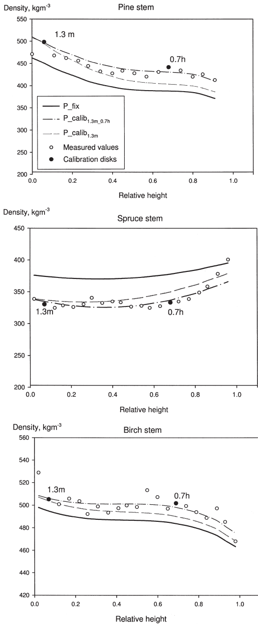
Fig. 5. Example of the predicted wood density in the vertical direction along birch, pine and spruce stems. P_{fix} are the predictions of the fixed part of Eqs. 4, 5 or 6. P_{calib1.3m_0.7h} and P_{calib1.3m} are the predictions (Eqs. 4, 5 or 6), which have been calibrated with random parameters using one or two sample disk measurements.
