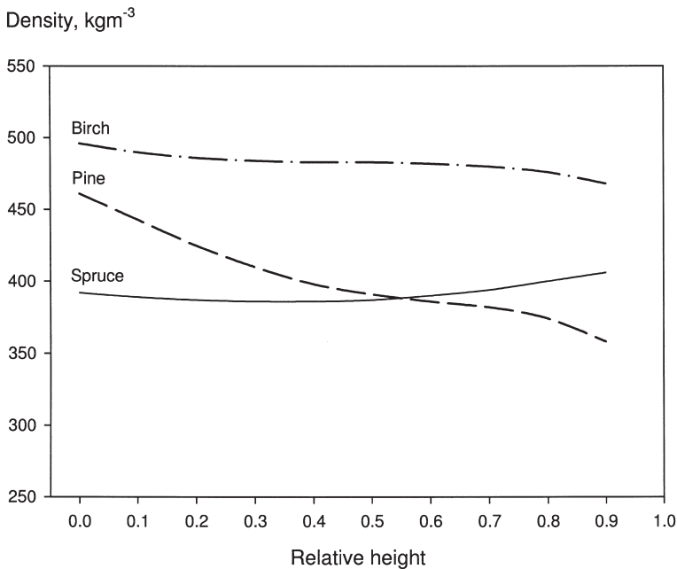
Fig. 4. Example of fixed predictions of wood density in the vertical direction along birch, pine and spruce stems according to models 4–6 ( h = 18 m and d_k/t_k = 4 ).
