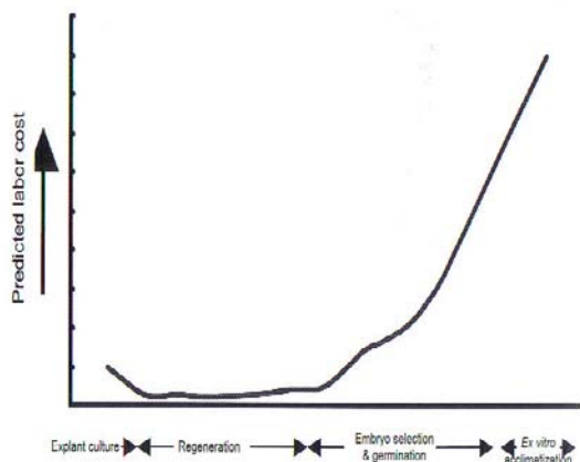
Fig. 1. Predicted labour cost by clonal propagation through somatic embryogenesis.
