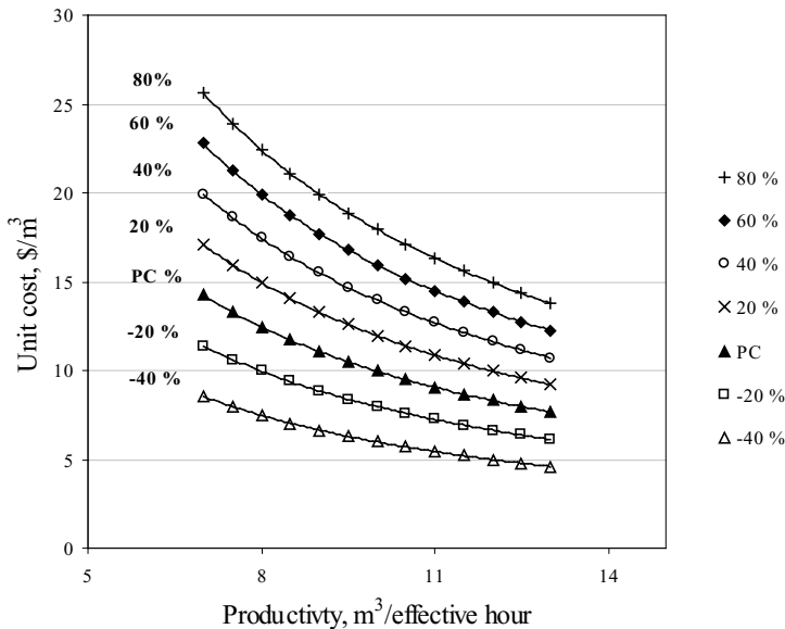
Figure 26. Sensitivity analysis of unit cost when the system cost of skidding changes by 20 % (PC = present condition).
