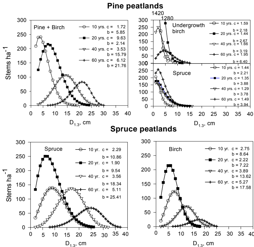
Figure 10. Mean DBH distributions of spruce and birch in drained spruce peatlands and pine peatlands (the dominant canopy layer of Scots pine and birch, and understorey spruce and birch) presented by drainage age classes. The Weibull parameters of each DBH distribution have been presented in the legends as examples.
